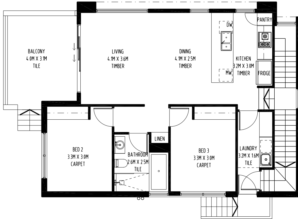
01 TOWN HOUSE 2 - LEVEL 2 PLAN - 1:100
