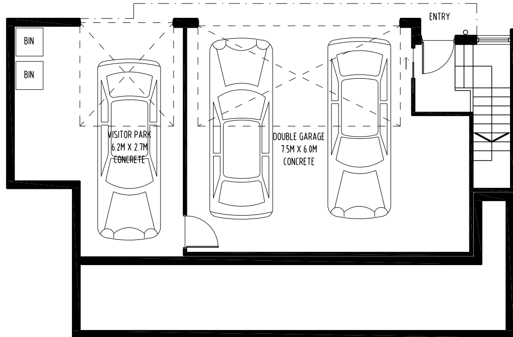
01 TOWN HOUSE 2 - LEVEL 1 PLAN - 1:100
